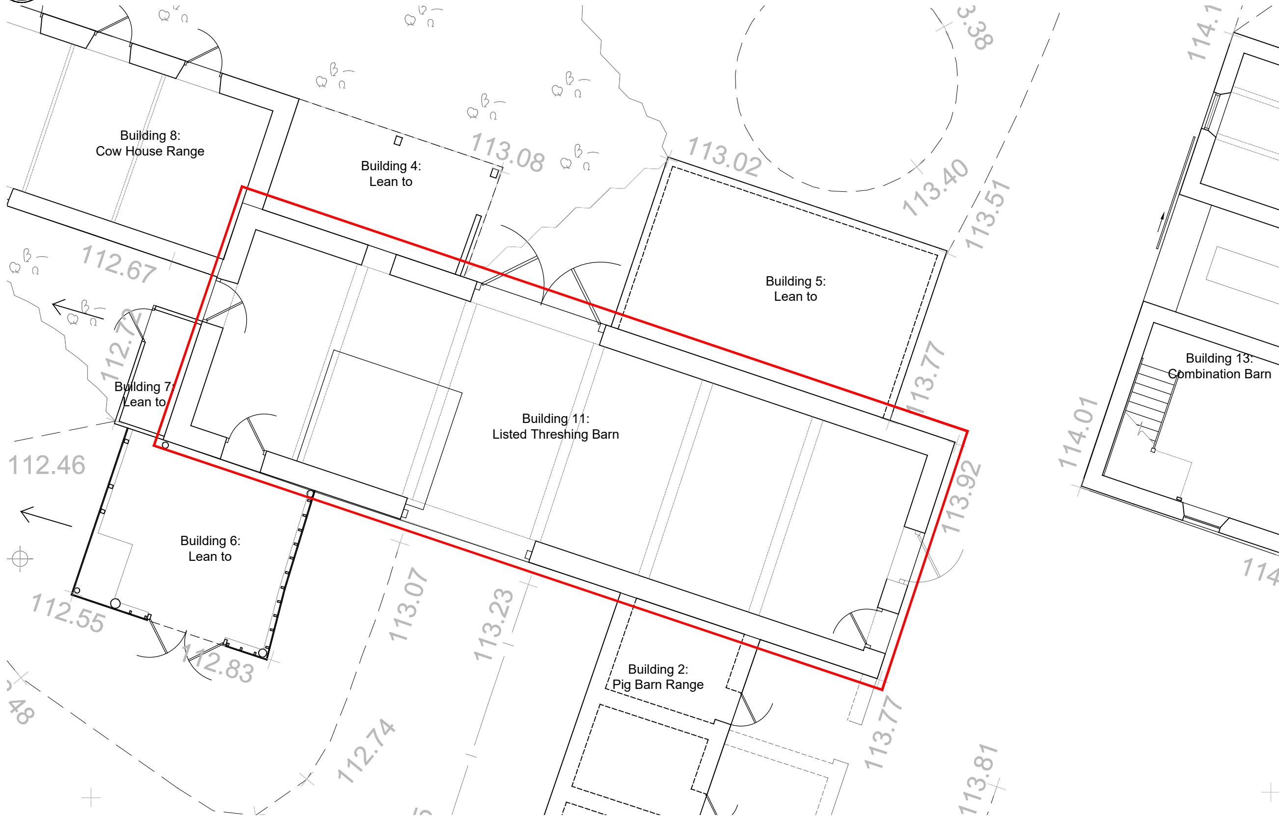
01 Ground Floor Plan, Listed Barn 1017 1:100
